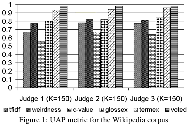
Figure 1: UAP metric for the Wikipedia corpus
