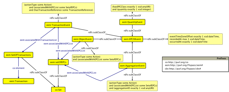
Fig. 3. EPCIS event classes as represented in EEM
